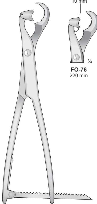
LAMBOTTE FO-50/FO-53 330 mm
