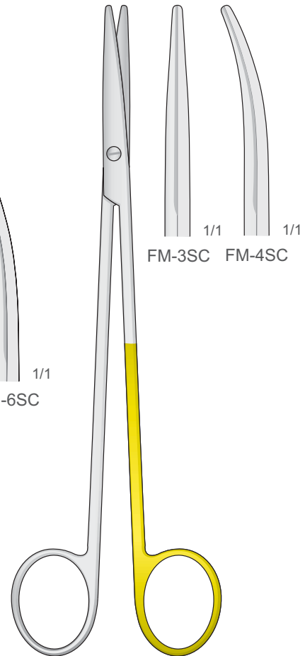
METZENBAUM FM-3SC/FM-4SC 185 mm
