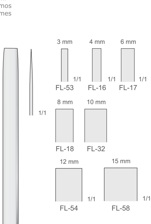
MINI-LAMBOTTE FL-16/FL-58 125 mm
